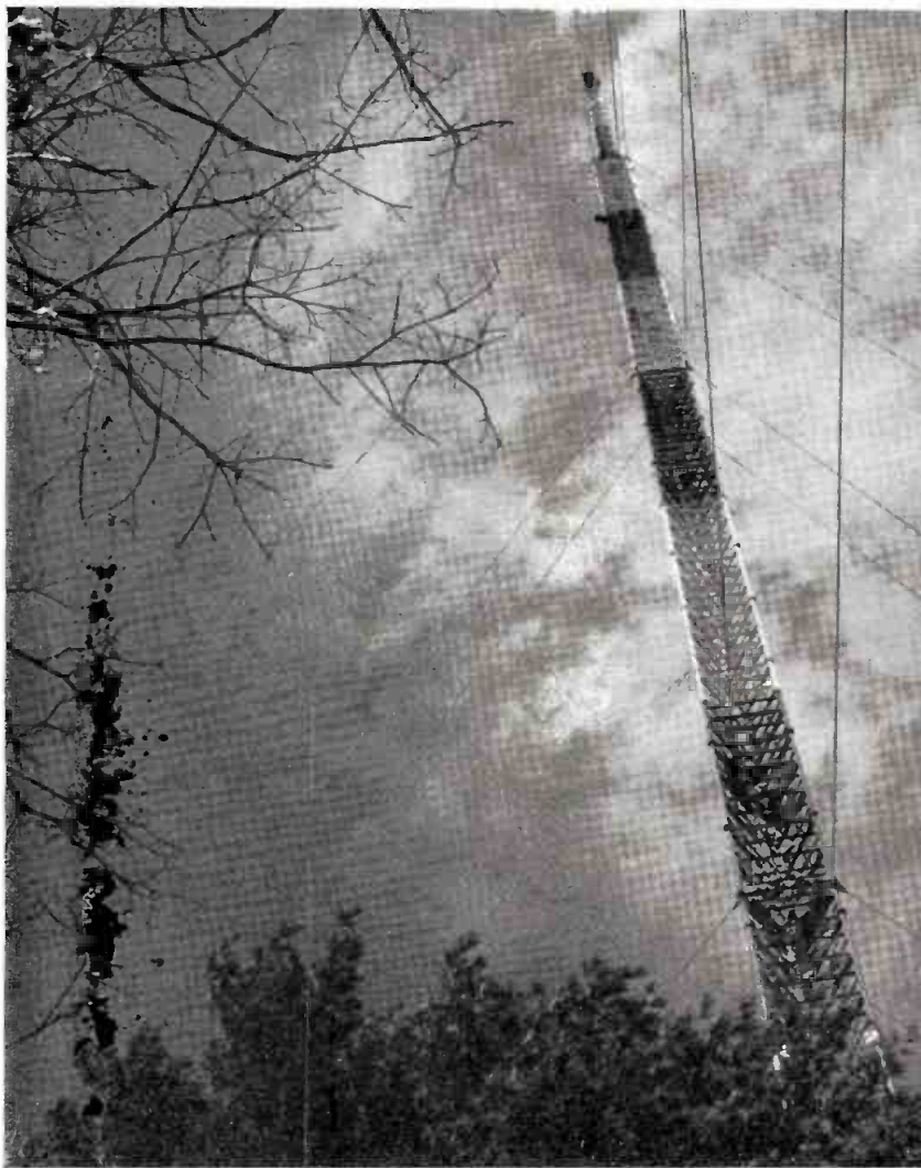
above—WBZ-TV's new Ideco tower at Boston, 1,199 feet above ground (1,349 feet Mean Sea Level). right—Slot antenna will side-mount directly beneath WBZ-TV's present antenna. The super-gain antenna will bolt into the bottom section of the narrow tower top.
