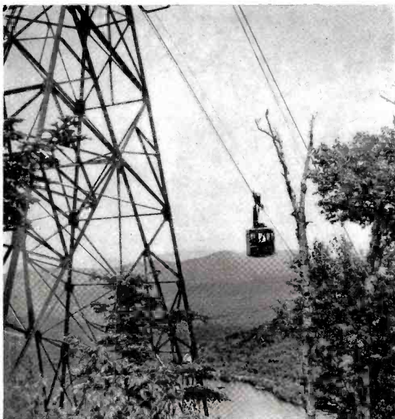
You'll Float Through The Air—For A Mile. This is a cable tramway for tourists that goes up Cannon Mountain at Franconia Notch in New Hampshire. The heavy wire ropes are well over a mile long, 1\frac{3}{4} inch in diameter and they weigh 28 tons apiece. The cable was made and installed by American Steel & Wire Division of United States Steel.
